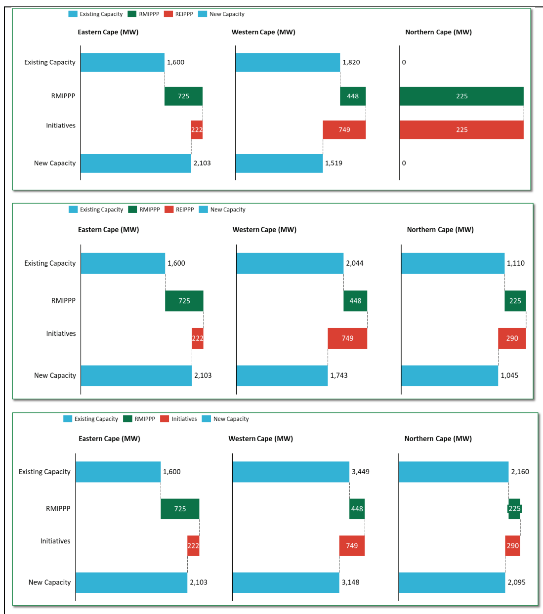
Figure 12: Grid capacity availability in the Cape in 2024, 2027 & 2028
