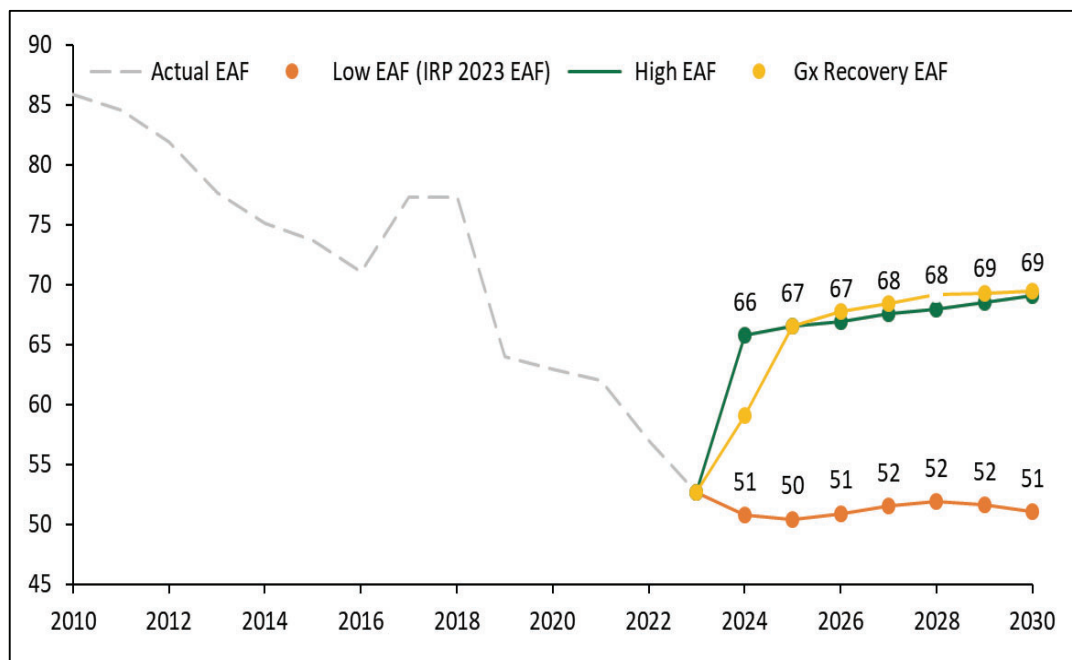
Figure 3: Overview of existing fleet EAF assumptions (%)
