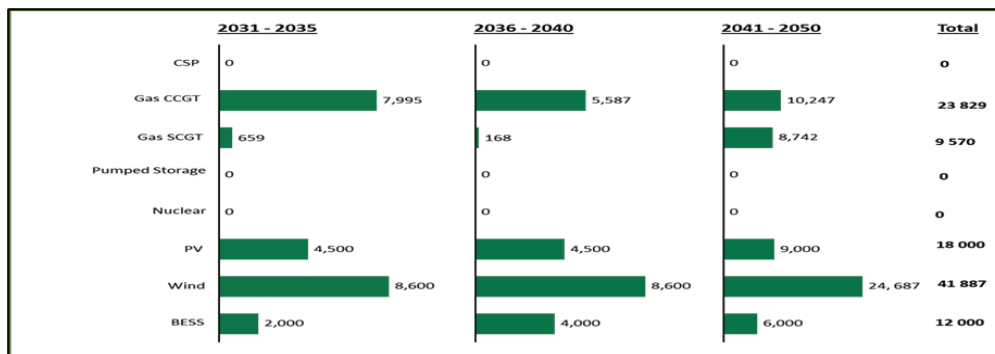
Figure 13: Reference Energy Pathway new generation capacity
