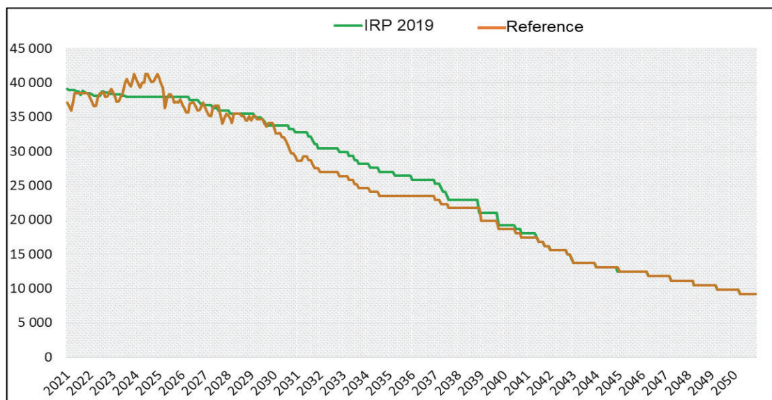
Figure 4: Overview of shutdown impact on existing coal-fired fleet installed capacity
