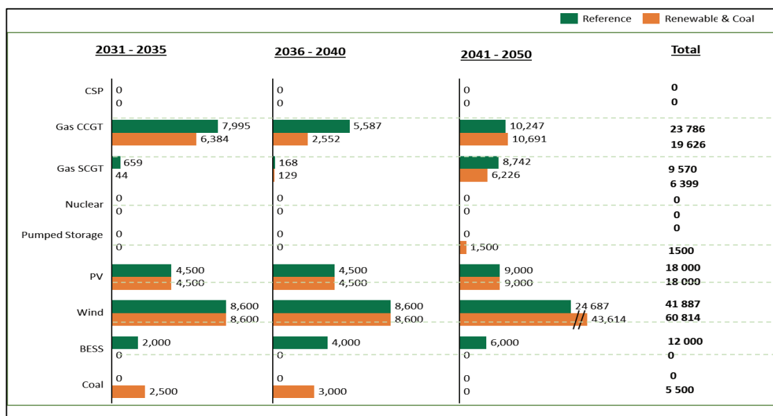
Figure 18: Pathway Six results
