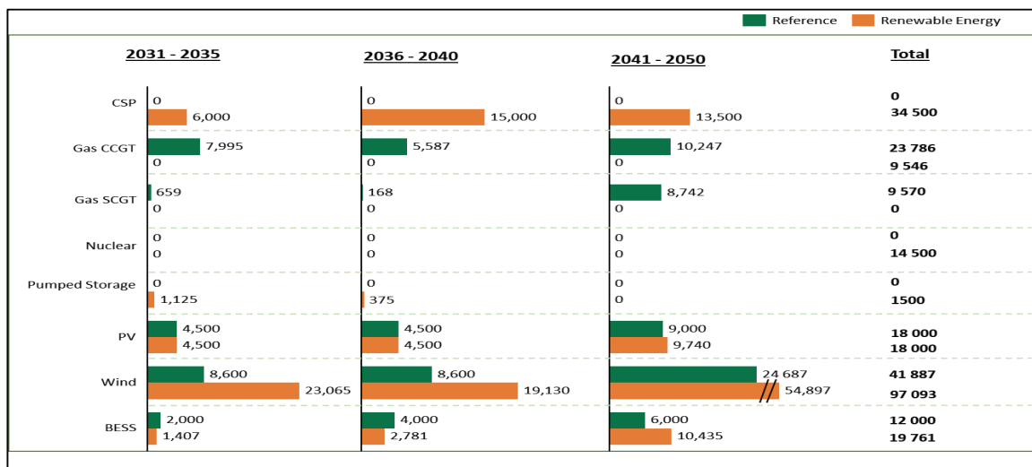
Figure 14: Pathway Two results
