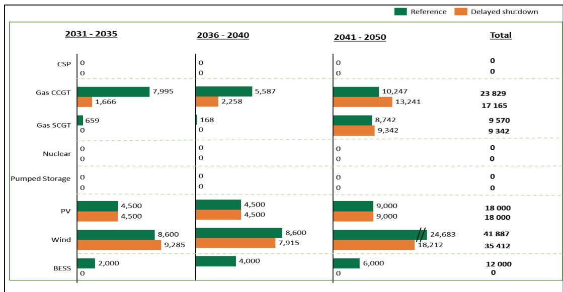
Figure 17: Coal Delayed Shutdown Pathway New Build Plan
